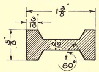
SECTION O-O
